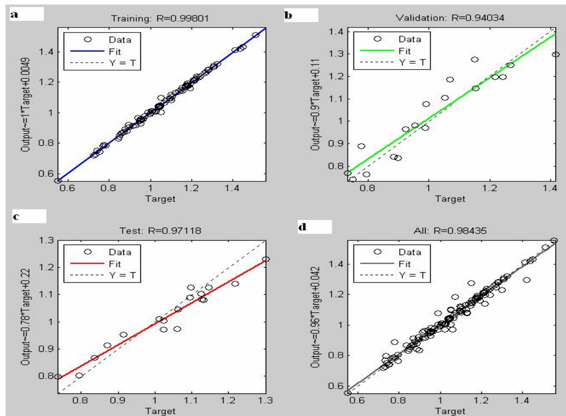
Figure 8 Accuracy of ANN for curl size estimation in the training phase (a), validation (b), test (c) and total (d)
