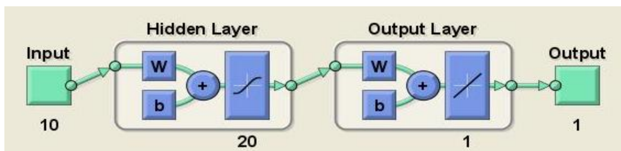
Figure 6 The ANNs structure for curl size estimation
