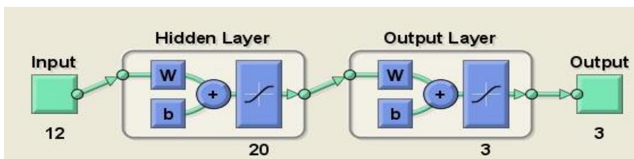
Figure 5 The ANNs structure for curl size classification
