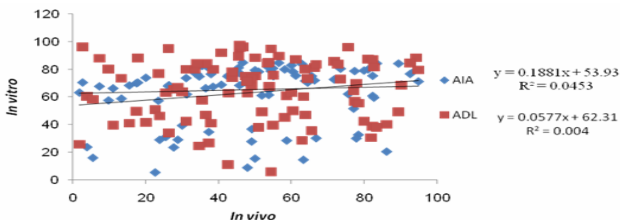
Figure 2 The correlation between in vitro and in vivo methods for digestibility of crude fat
